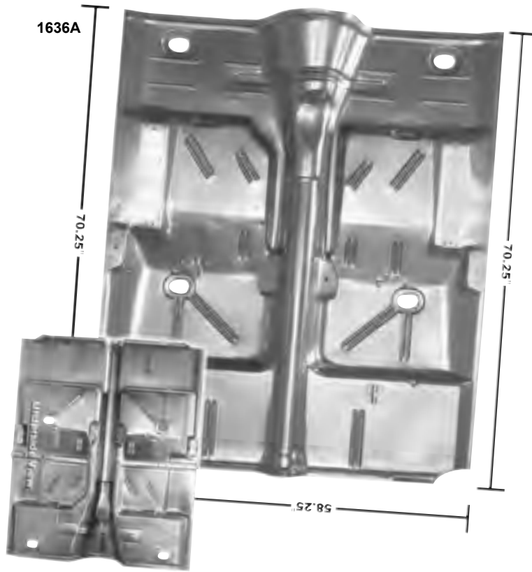
1636A 1962-67 Complete Floor Pan (no hole) MSRP $477.00 ea 1636B 1962-67 Floor Cover, For Manual Transmission MSRP $45.00 ea
